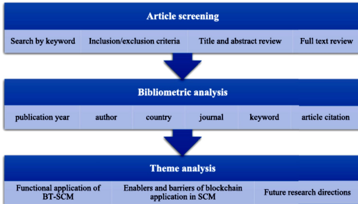
Figure 1. Review process
